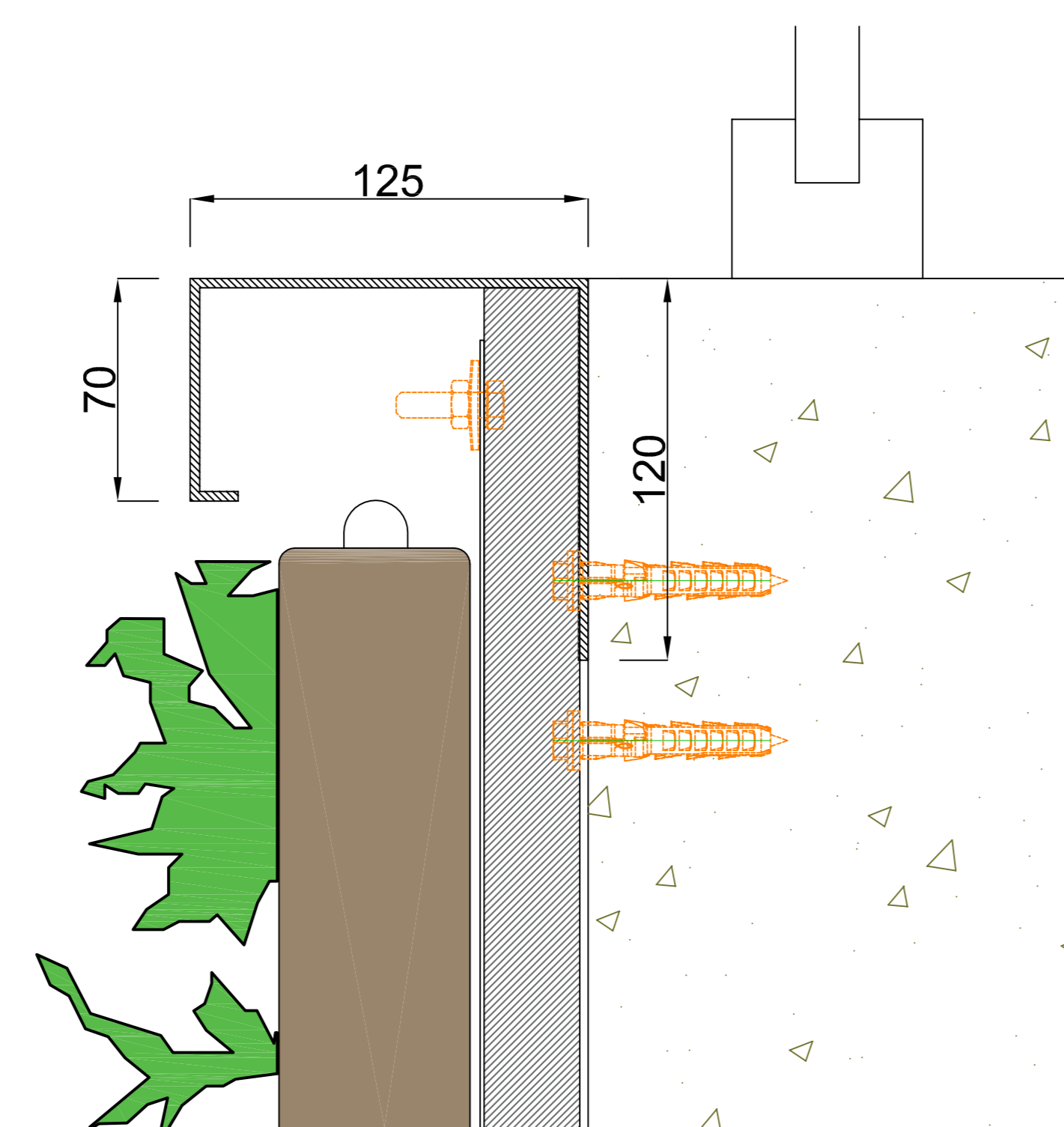
Detail 2 1:5
