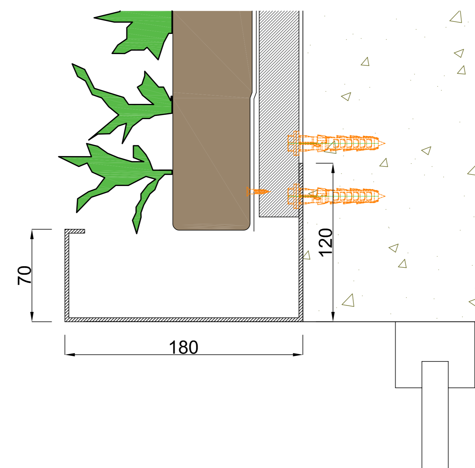
Detail 3 1:5
