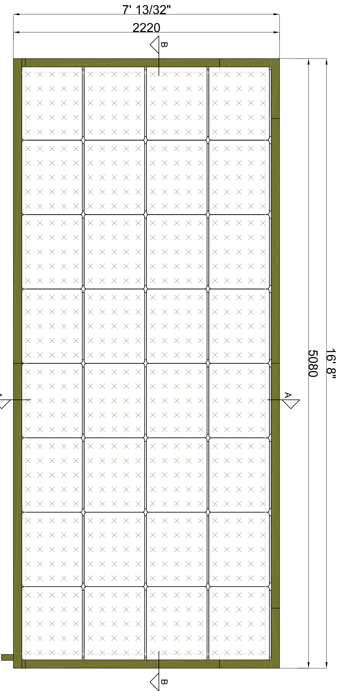
Front view
