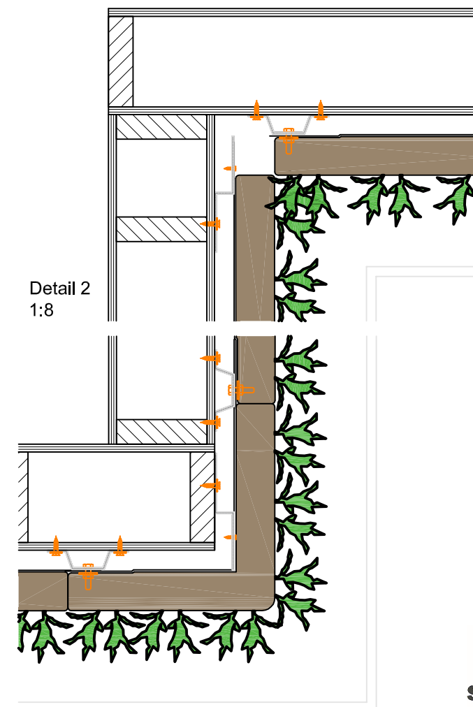
Detail 2 1:8
