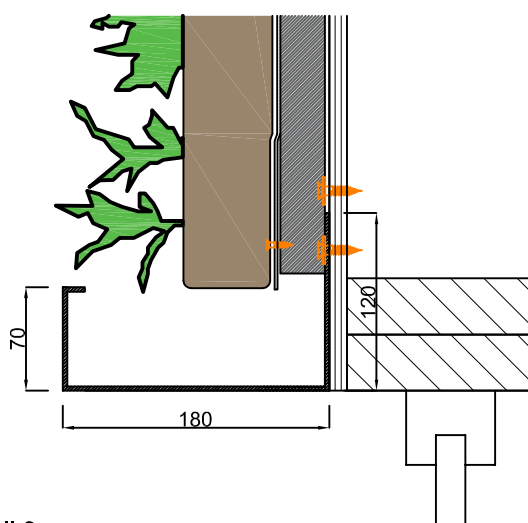
Detail 3 1:5
