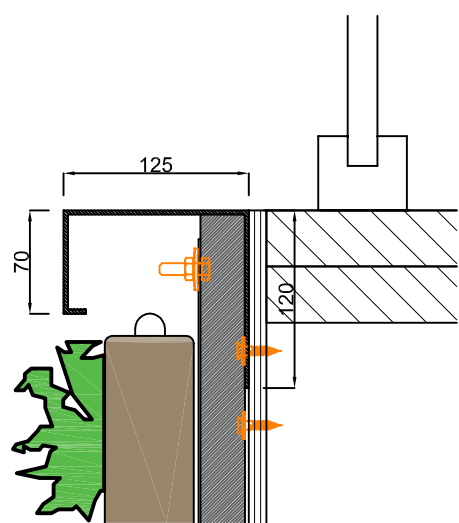
Detail 2 1:5
