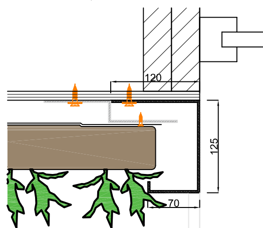
Detail 1 1:5
