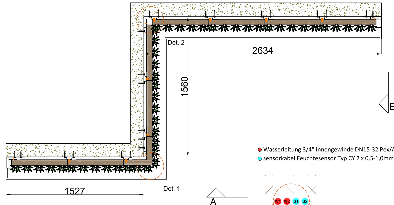
Detail A 1:8
